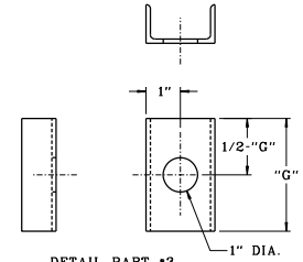
DETAIL PART #3 SCALE: 1/2" = 1"
