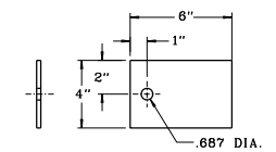
DETAIL PART #6 SCALE: 1/4" = 1"
