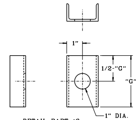
DETAIL PART *3 SCALE: 1/2" = 1"
