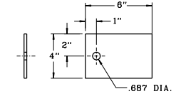
DETAIL PART #6 SCALE: 1/4" = 1"
